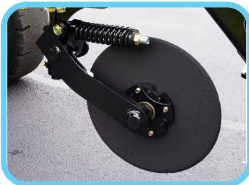
Spring loaded coultter blade
