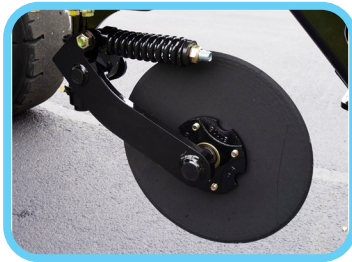
Spring loaded coulter blade
